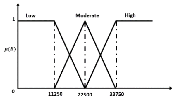
Fig 4. Membership degree function of CO
